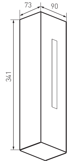
Power pack-Surface Mount
